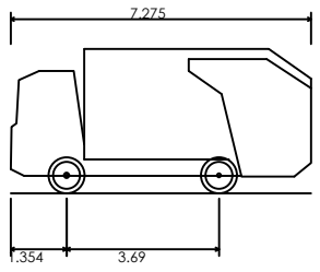
REAR LOADING COLLECTION VEHICLE URBIN
